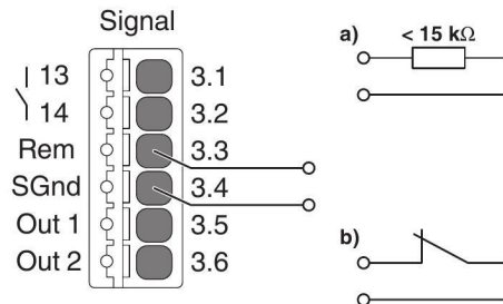
Figure 23 SLEEP MODE connection versions
