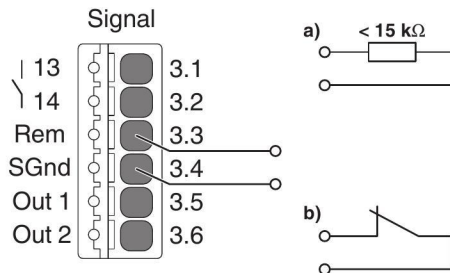
Figure 36 External wiring versions, enable SLEEP MODE
