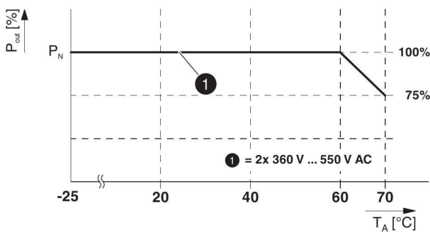
Figure 50 Output power in 2AC operation
