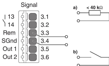
Figure 37 External wiring versions, disable SLEEP MODE
